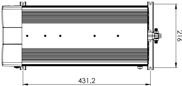
WP-Sine XFR 12/3000
